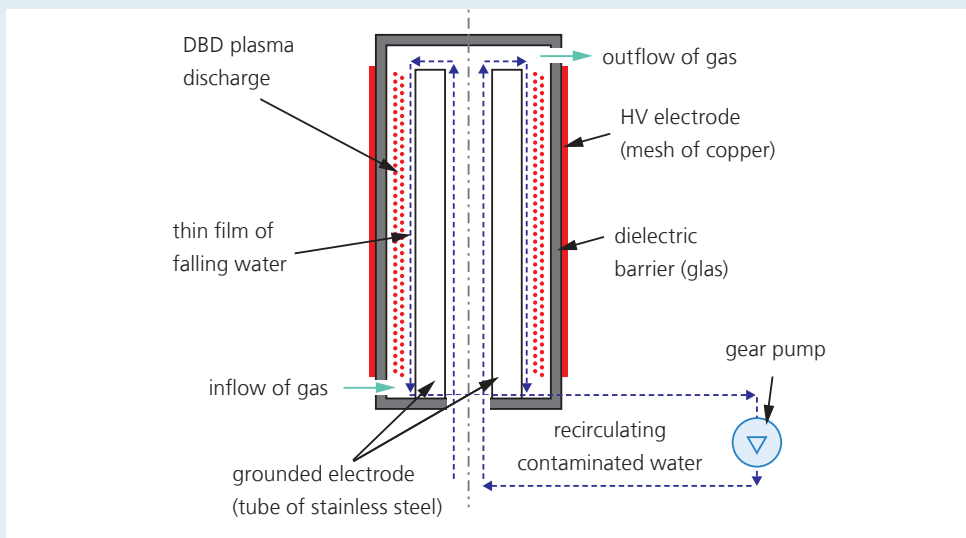
Schematic structure of a plasma reactor for water treatment.
